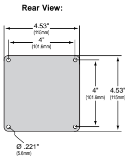
FX-30 Wall Mount Interface
