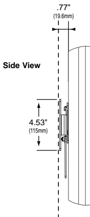
FX-30 Wall Mount Interface
